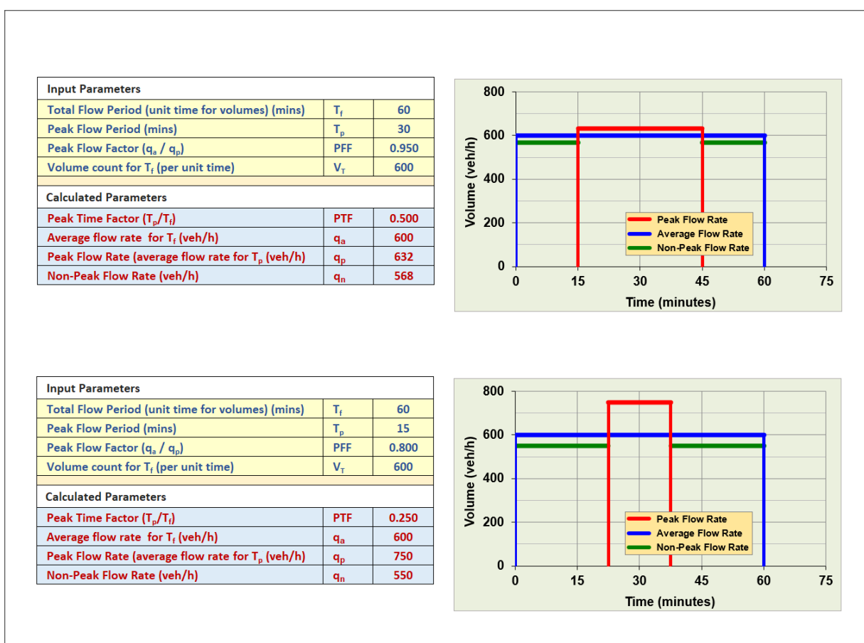
Figure 8 - Low peaking and high peaking examples
