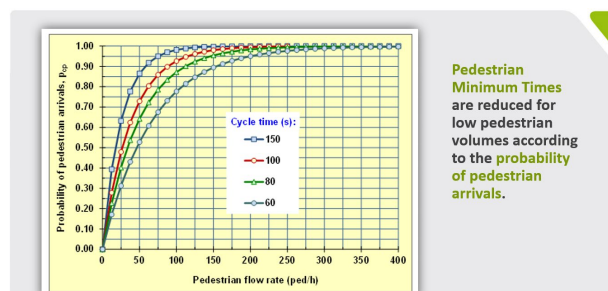
Figure 10 - Pedestrian analysis in SIDRA intersection modelling
