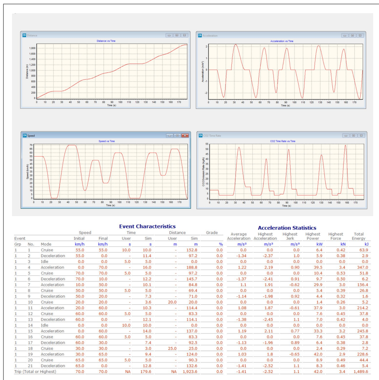
Figure 5 - Drive Cycles for detailed modelling of vehicle paths - an example from SIDRA TRIP
