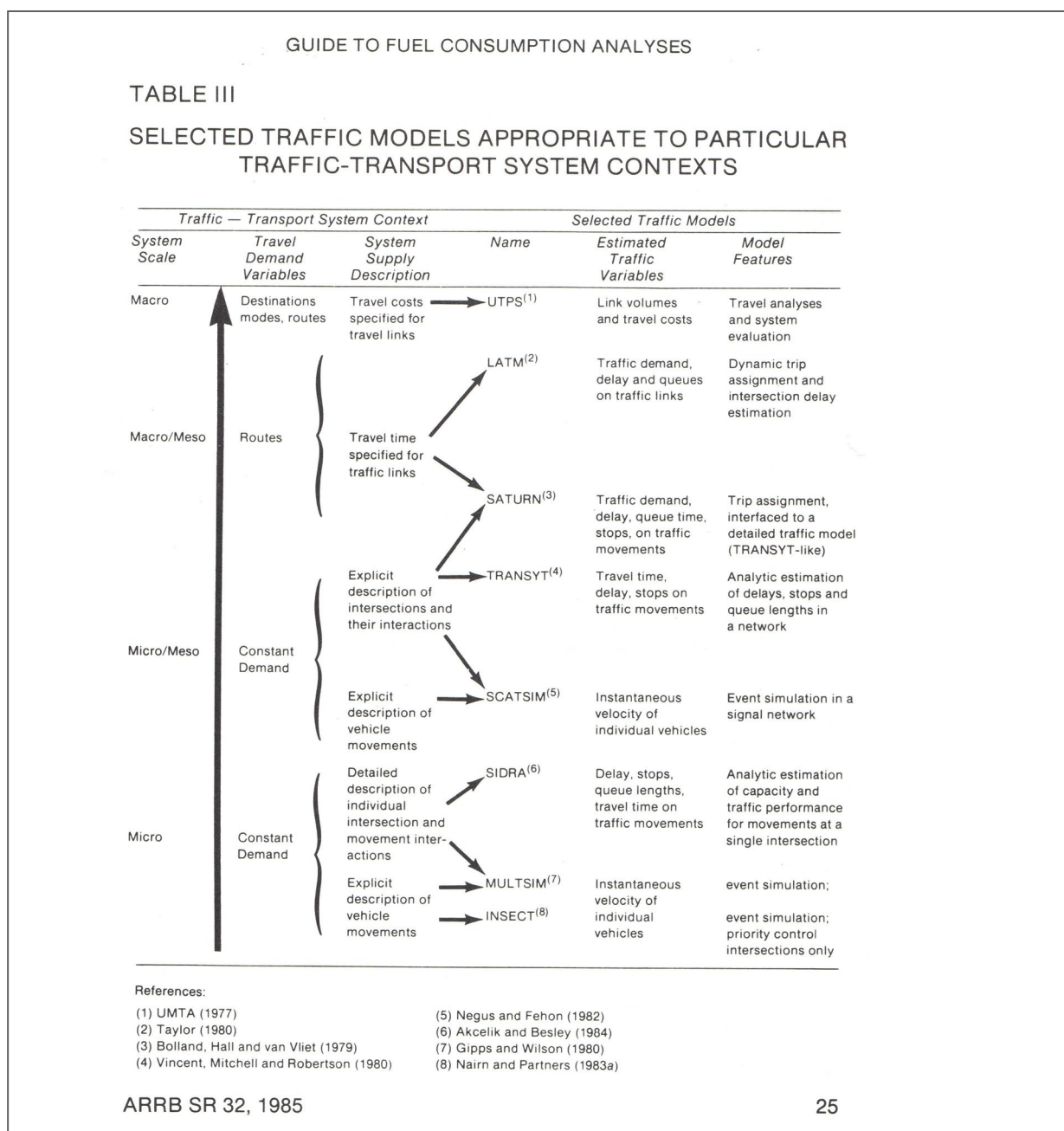
Figure B.1 - Traffic Model Hierarchy presented in ARRB Special Report 32 (Bowyer, Akcelik and Biggs 1985)
