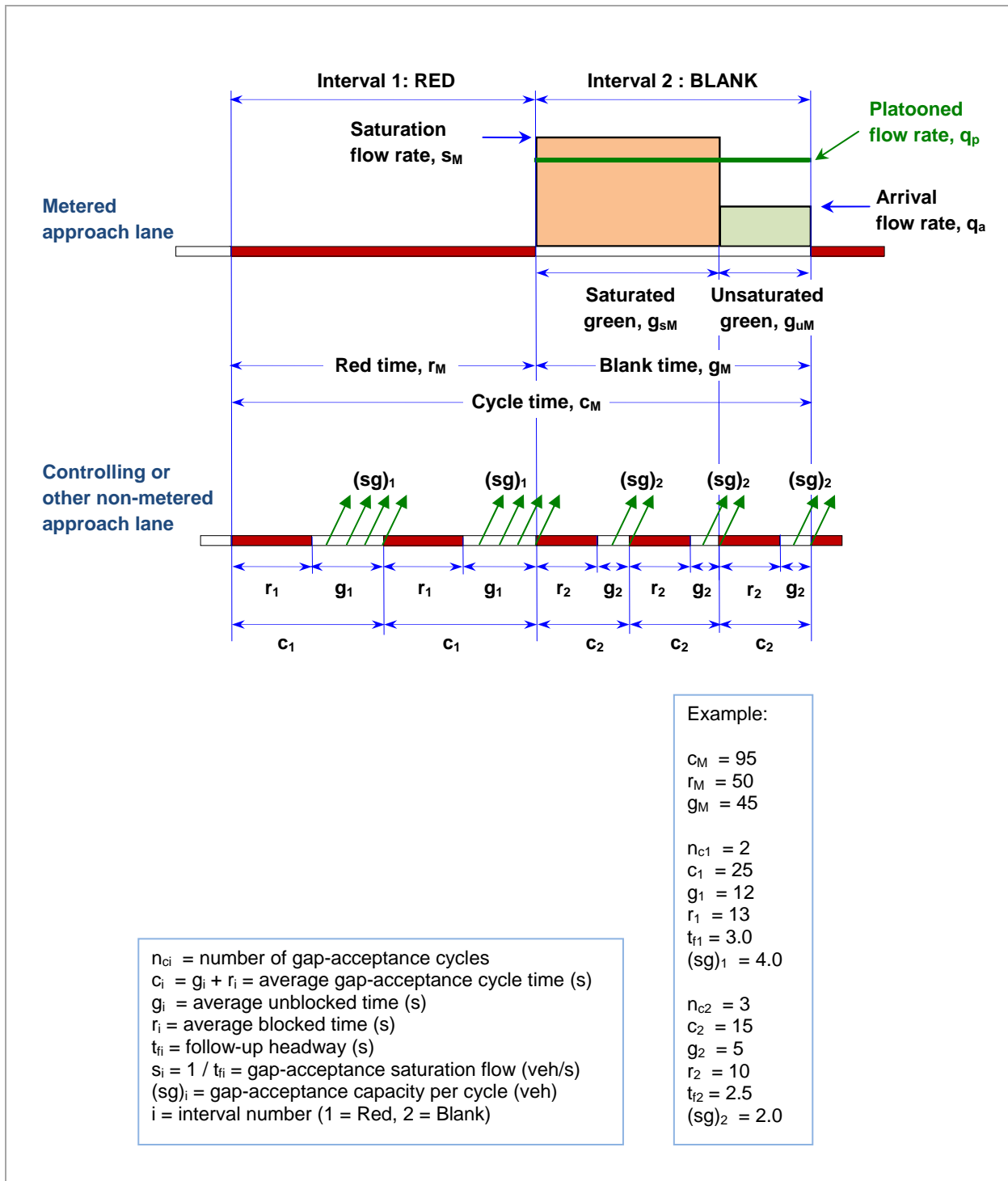
Figure 2 - The departure pattern and platooned arrival rate for a Metered approach lane during the Blank interval, and the gap-acceptance cycles for Controlling and other non-metered approaches during Blank and Red intervals
