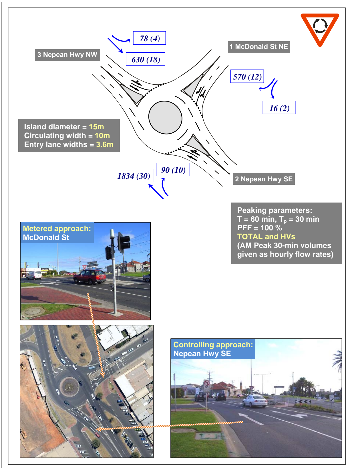
Figure 3 - Roundabout metering signals case study: Nepean Highway - McDonald Street, Mordialloc, Victoria, Australia
