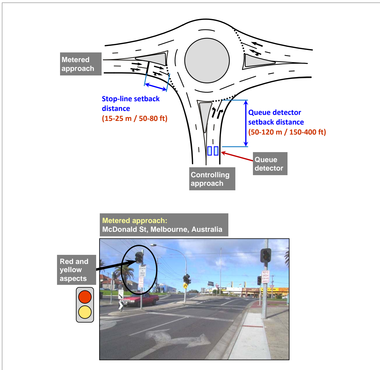
Figure 1 - Roundabout metering signals
