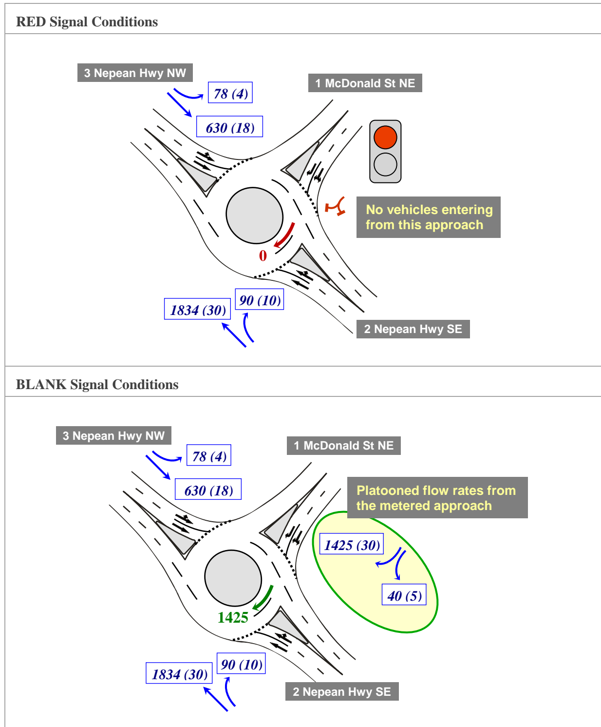
Figure 4 – Modeling of Red and Blank signal conditions
